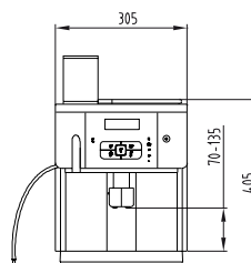
Schaerer Coffee Joy with bean hopper extension
